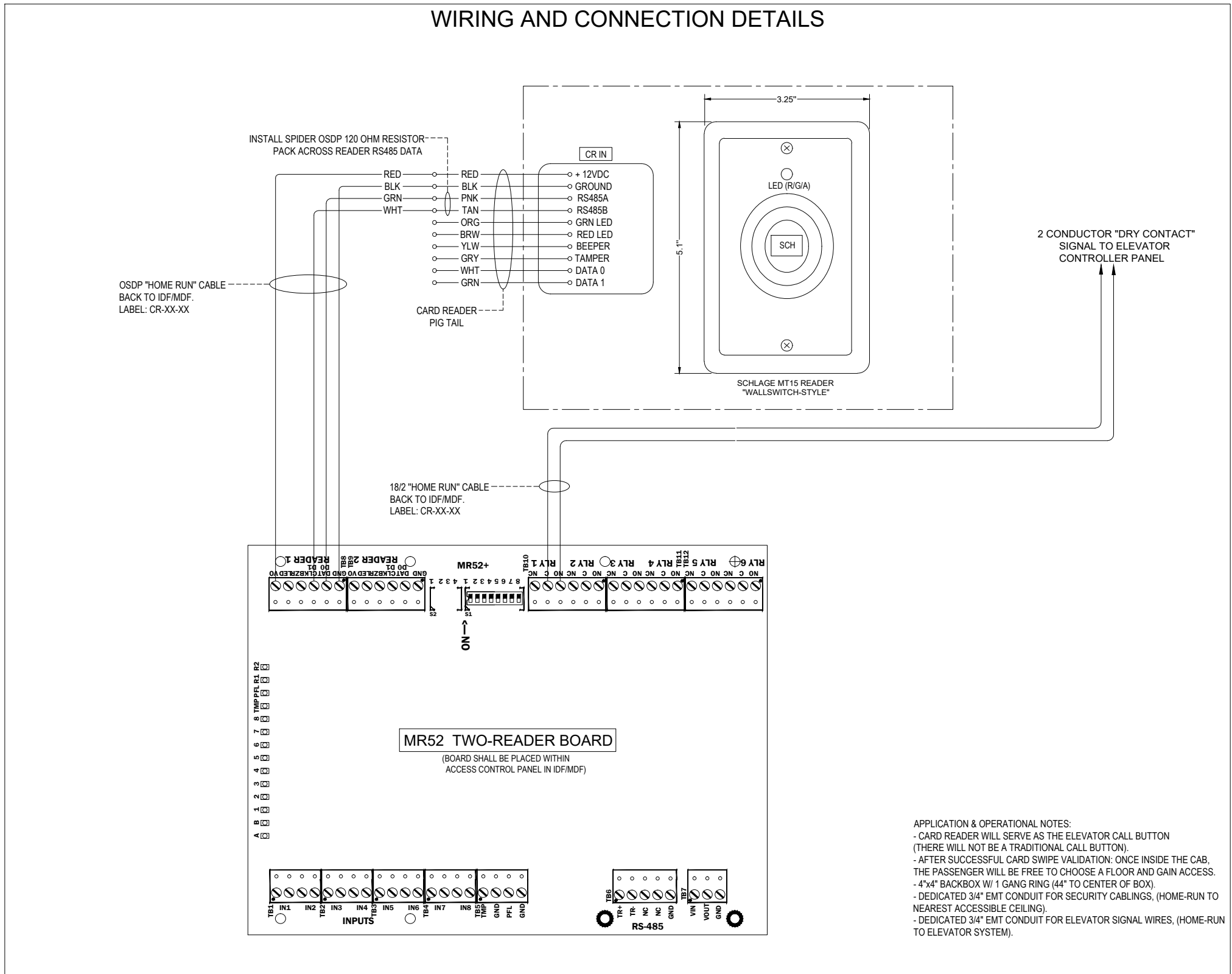
4 TYPICAL ELEVATOR HALL CALL CARD READER (CR)
