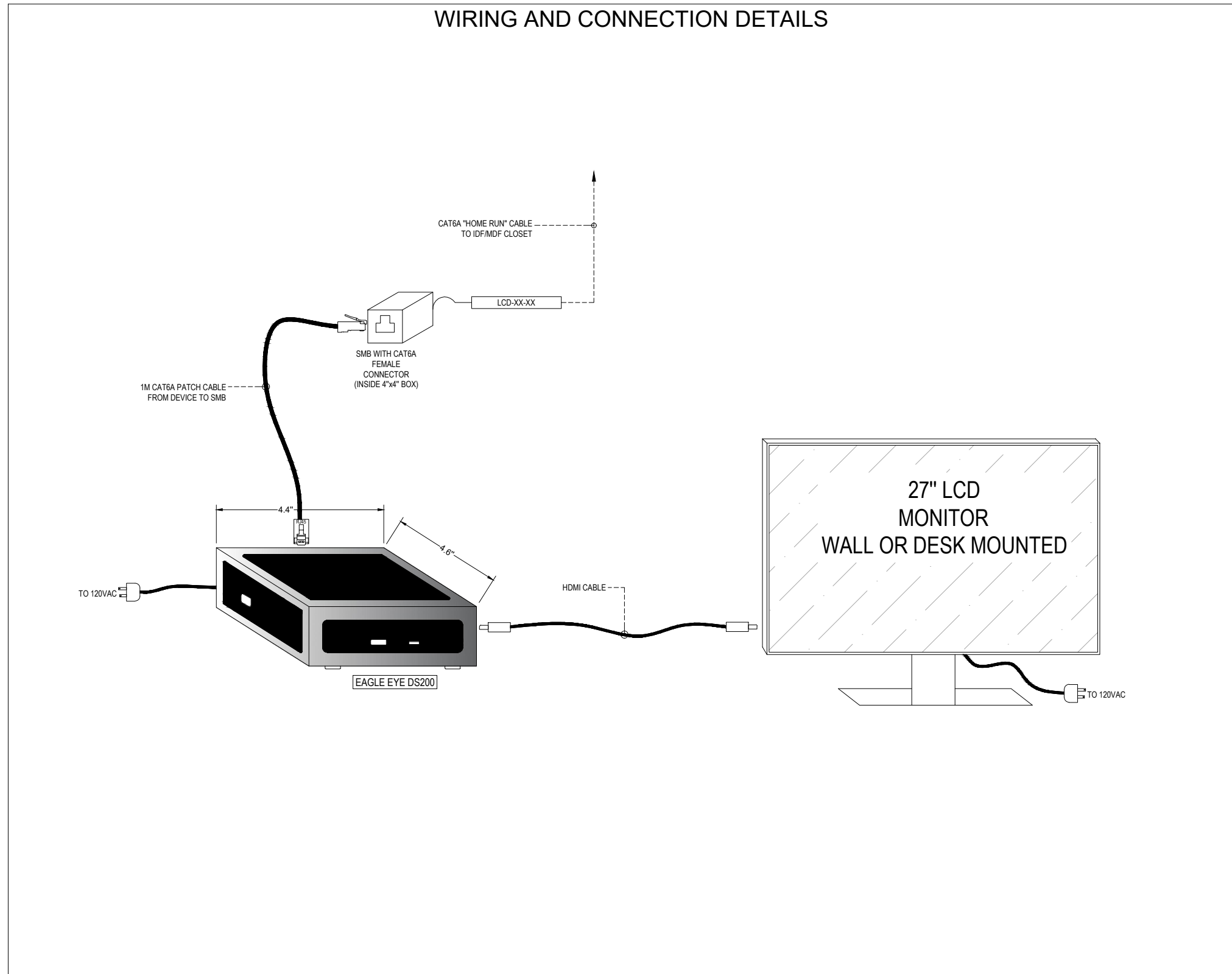
3 TYPICAL FIELD LCD MONITOR CAMERA DISPLAY (LCD-XX-XX)
